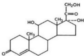
Figure 2: Structural Formula of Hydrocortisone
